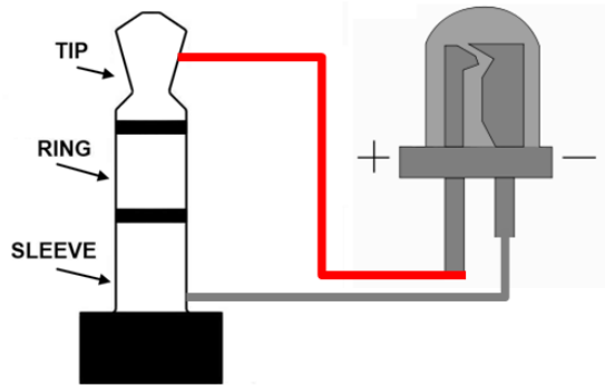
TRS Connector IR LED 圖 2-8、TRS 接頭連接 IR LED
