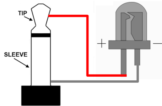
TS Connector IR LED 圖 2-9、TS 接頭連接 IR LED
