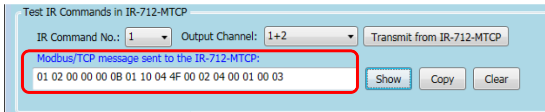
Figure 4-1 Test IR commands stored in IR-712-MTCP
