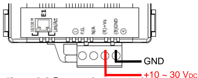
Figure 2-3 Power wire connection
