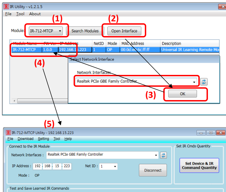
Figure 2-4 Steps of connecting the IR-712-MTCP
