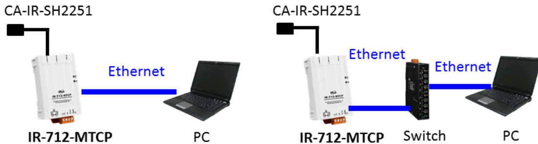
Figure 2-2 Communication wire connection between the IR-712-MTCP and PC
