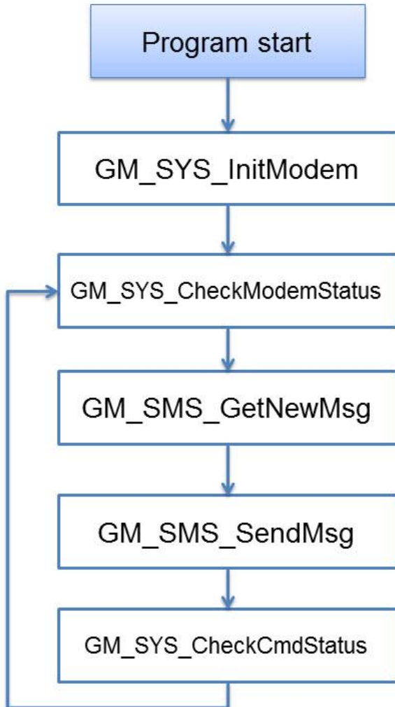
SMS Design Flowchart
