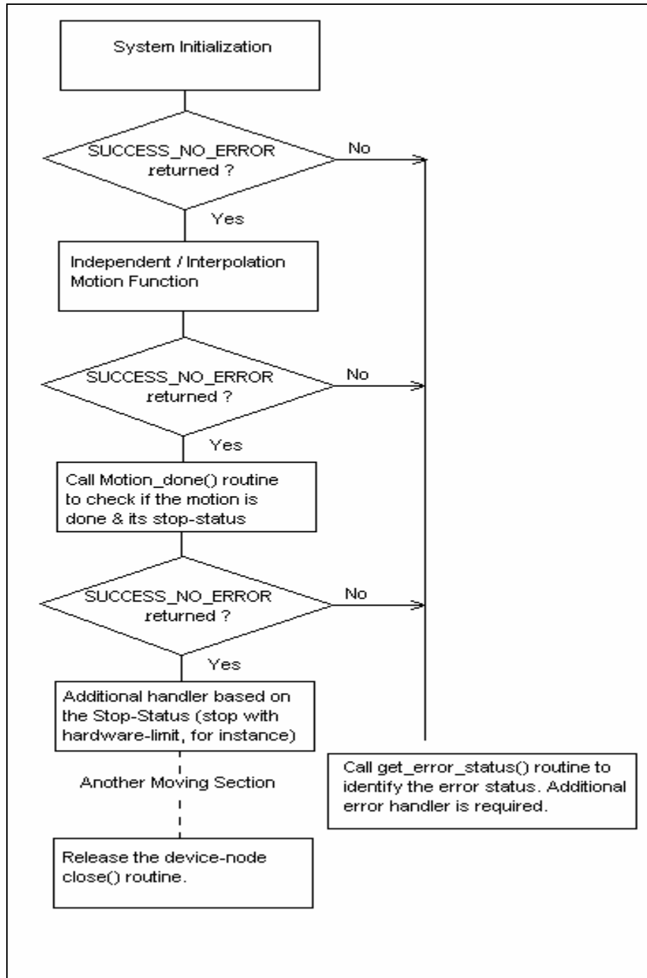
Figure 1 - typical programming follow-chart
