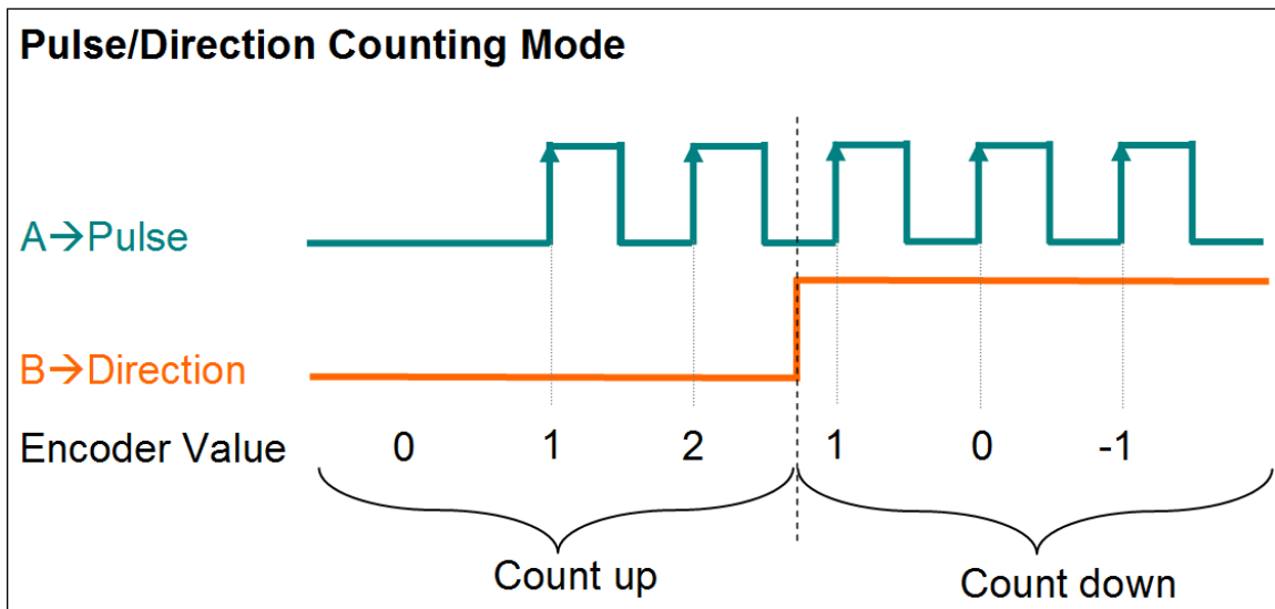
圖 23: Pulse/Direction counting mode
