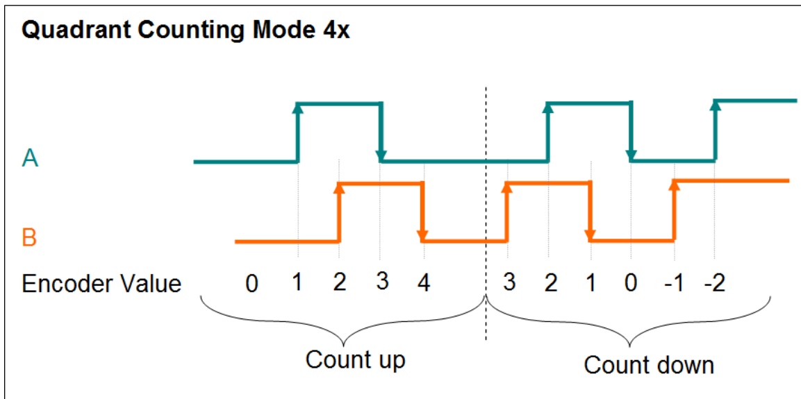
圖 25: Quadrant counting mode
