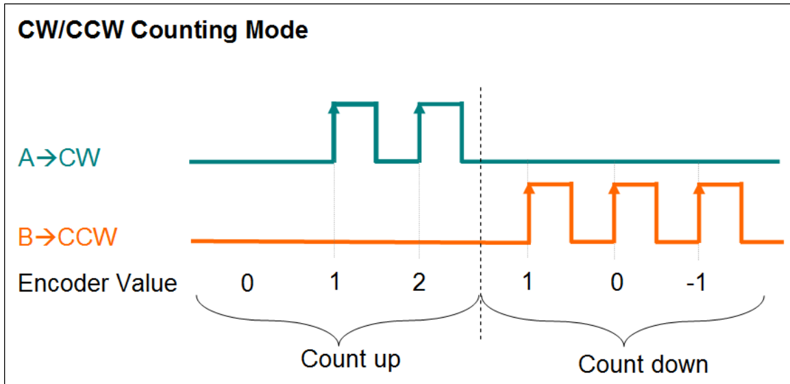
圖 24: Clockwise/ Counterclockwise counting mode
