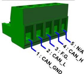
5-pin screw terminal block
