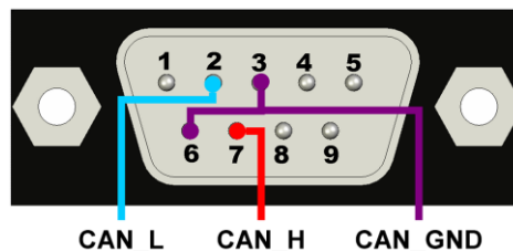
9-pin D-Sub male connector
