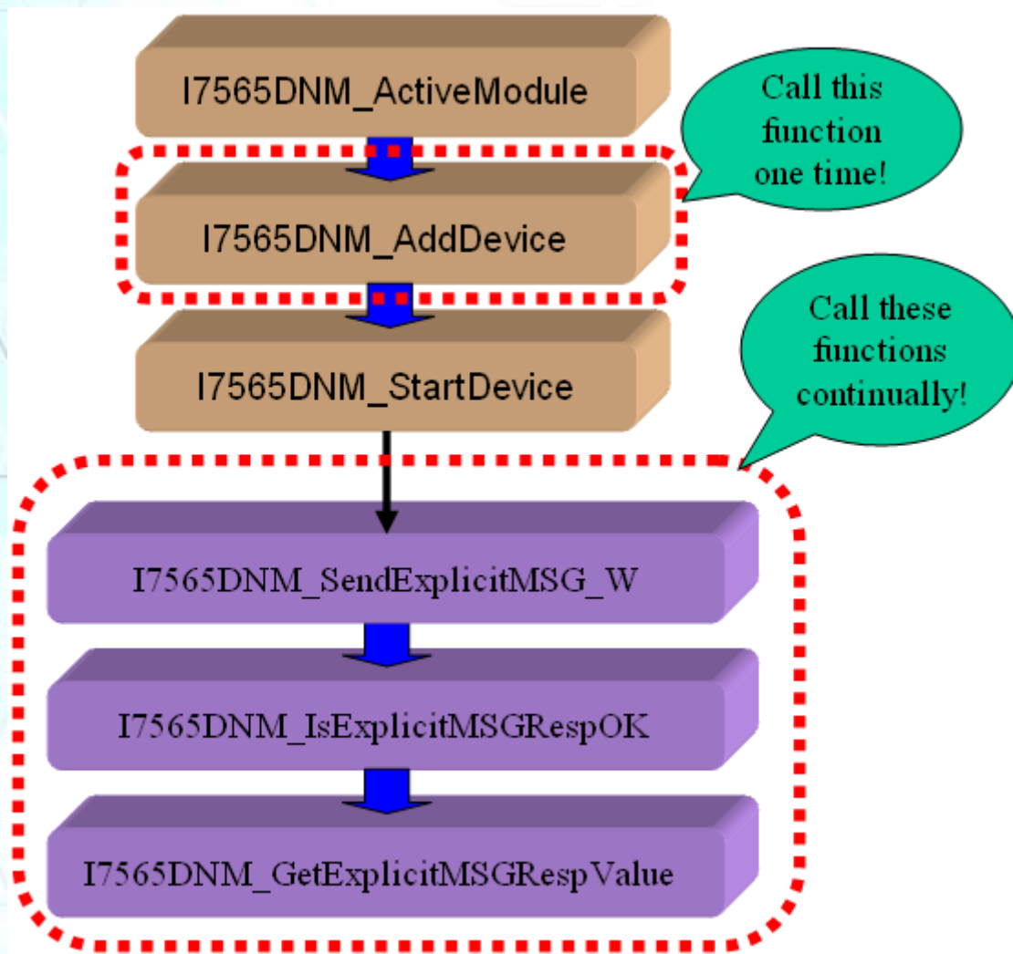
Figure 3.9 “SendExplicitMSG_W” Diagram
