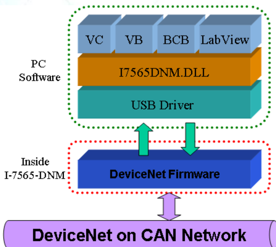
Figure 1.2 I-7565-DNM architecture.
