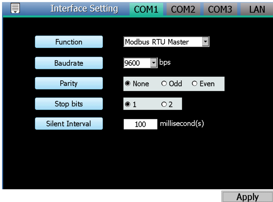
Figure4-2: Interface Setting page (Com Port)
