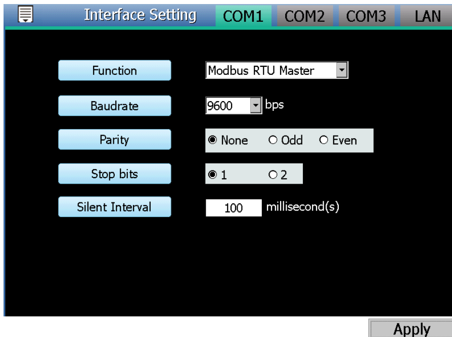
Figure4-3: Function setting to connect to Modbus RTU slave module
