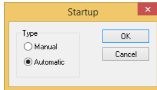
Startup dialog
