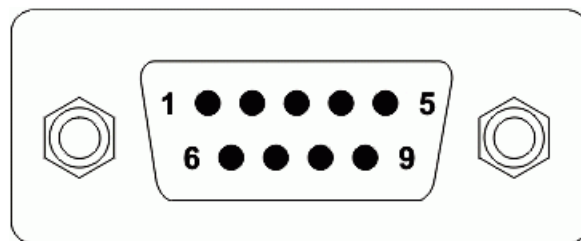
DB9-Male (COM1)
